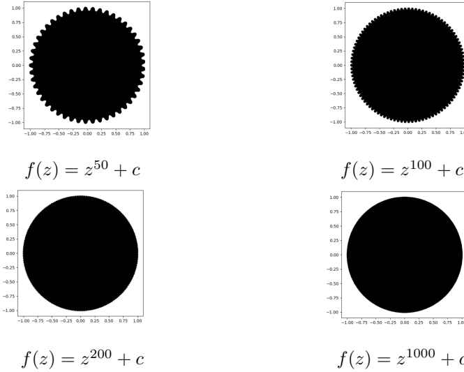
Figure 3: Representative Multibrot sets for f(z) = z^j + c . As the degree increases, the sets become increasingly circular and their boundaries progressively smoother. Images were generated using Python’s NumPy and Matplotlib libraries on a 1000 \times 1000 grid with an escape-time algorithm using 200 iterations.
